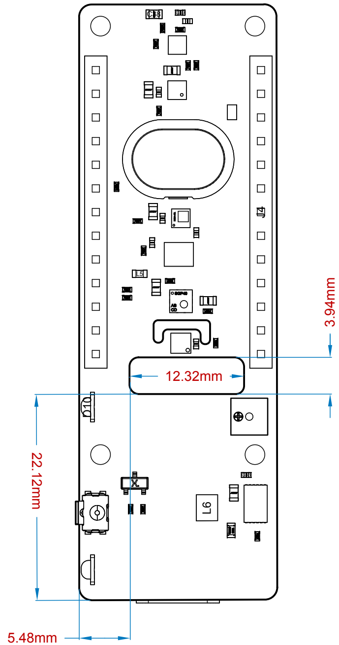
View from Bottom side (Scale 5:2)
