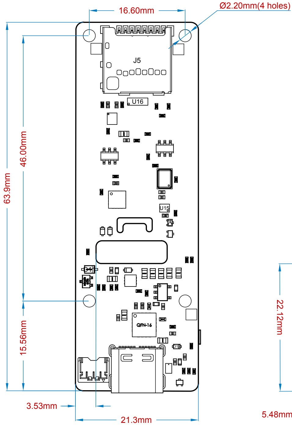
View from Top side (Scale 5:2)
