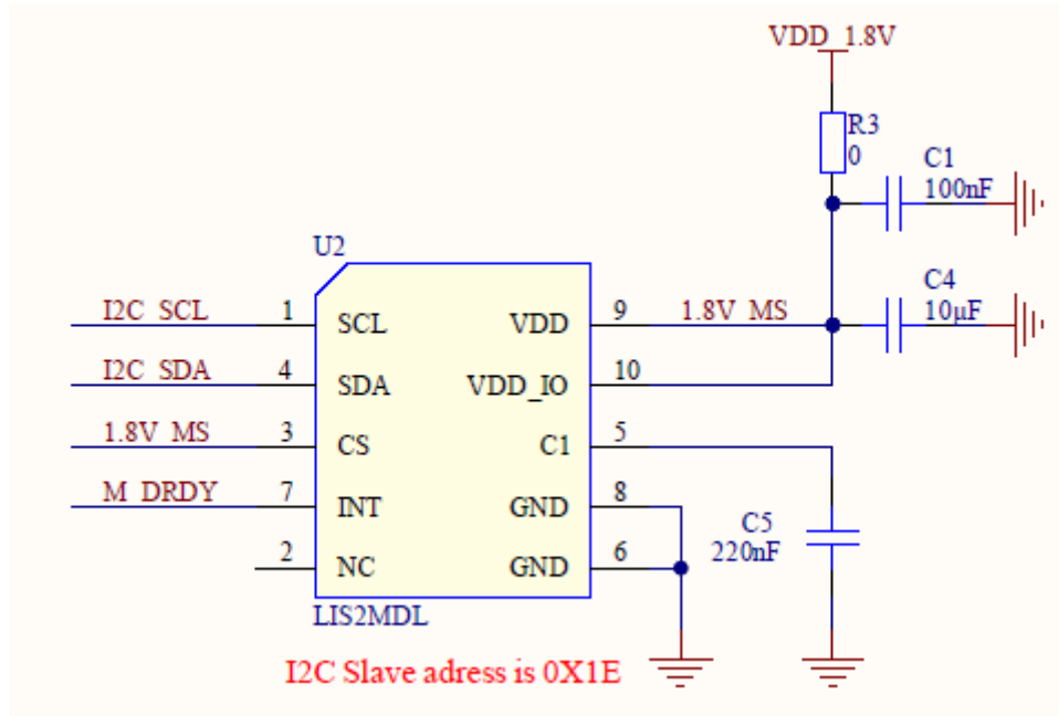
Figure 7. LIS2MDL connection
